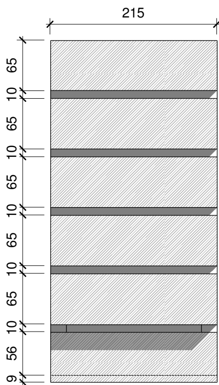
Front Elevation
