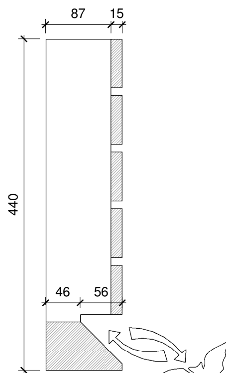
Side Elevation
