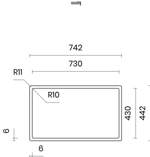
FILOTOP Flushmount
