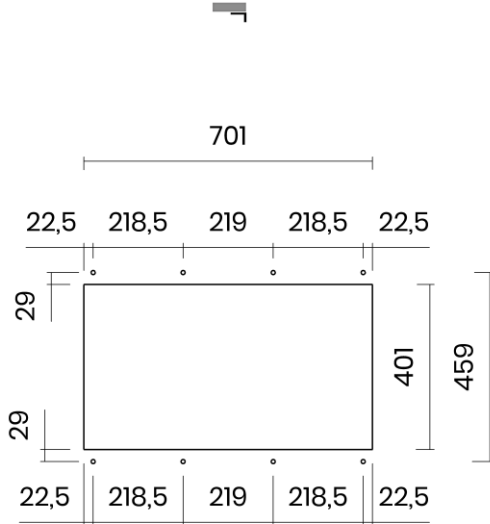
SOTTOTOP Undermount
