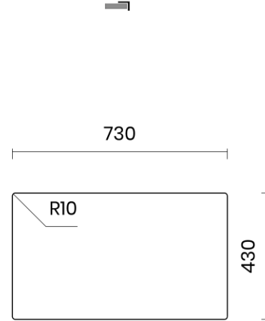
SOPRATOP Topmount
