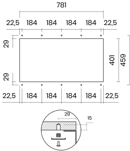
FILOTOP Flushmount
