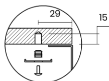
FILOTOP Flushmount
