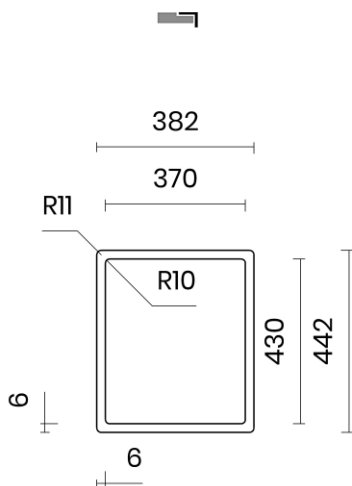
FILOTOP Flushmount
