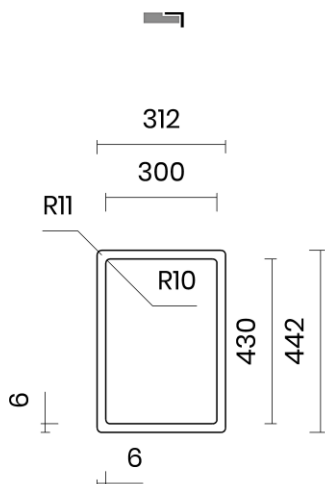
FILOTOP Flushmount
