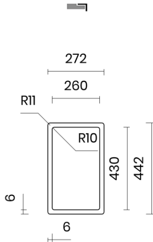
FILOTOP Flushmount
