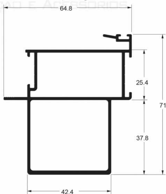
SU-290 1,247 Kg/m
