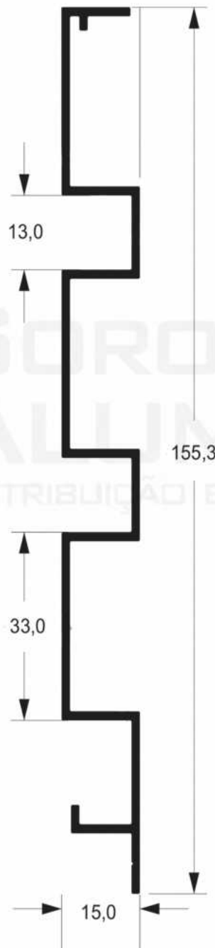
DP-017 1,079 Kg/m
