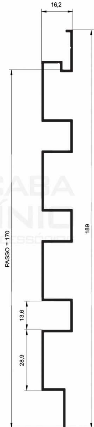
DP-018 1,028 Kg/m
