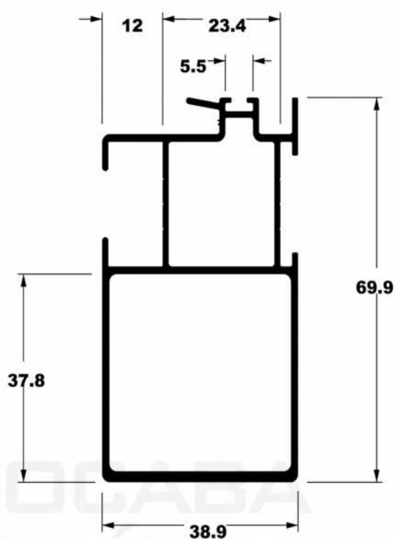
SU-290 1,247 Kg/m
