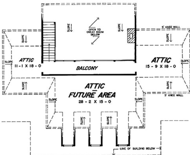
FUTURE SECOND FLOOR PLAN
