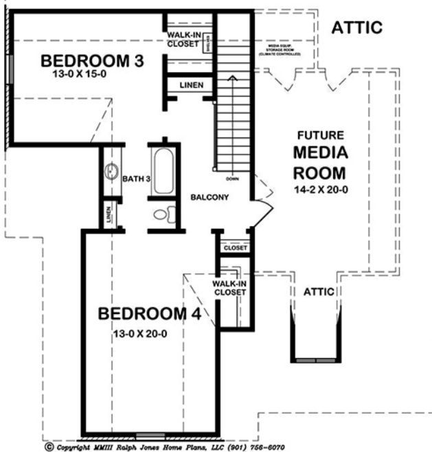
SECOND FLOOR LAYOUT
