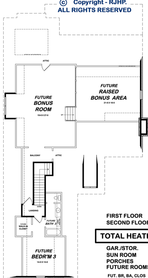
FUTURE SECOND FLOOR PLAN
