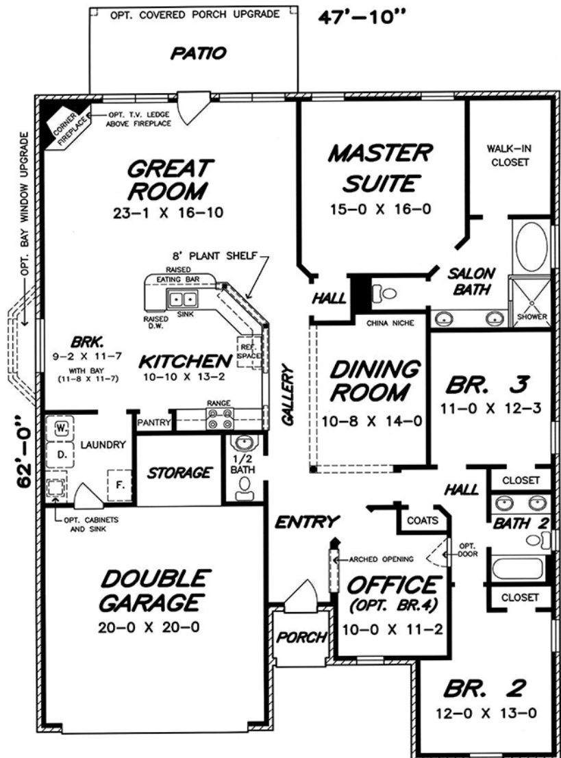
OPT. PLAYROOM / OFFICE LAYOUT
