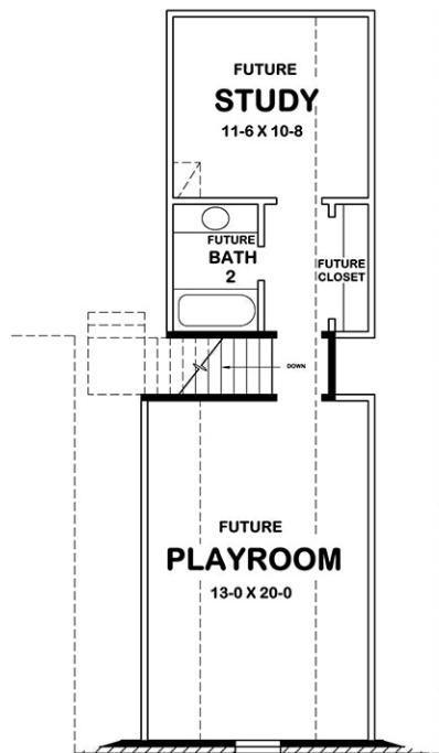
FUTURE Second Floor Plan
