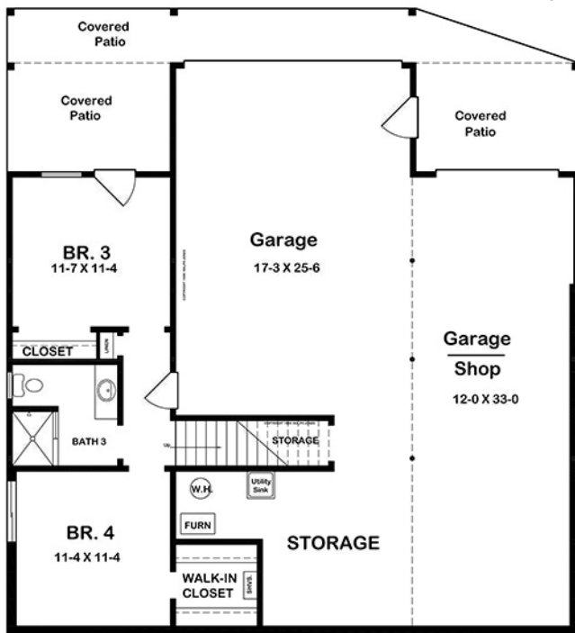
Lower Level Floor Plan
