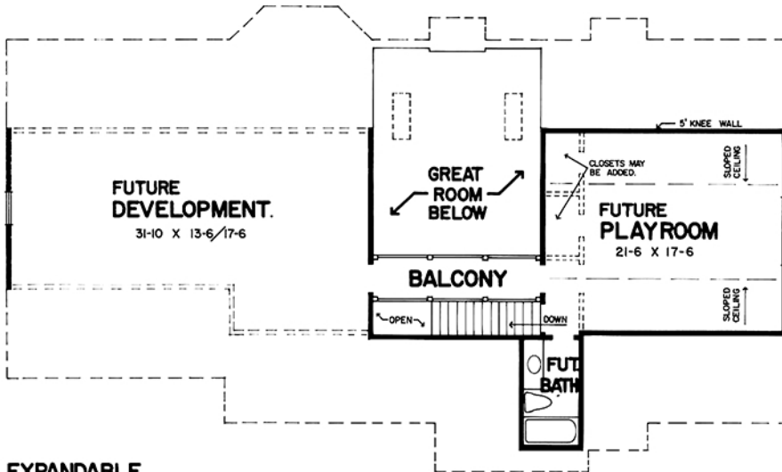
EXPANDABLE SECOND FLOOR PLAN
