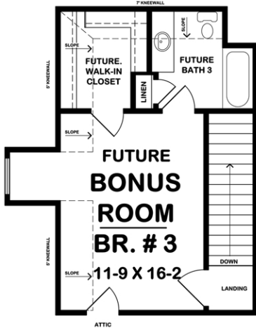
OPT. SECOND FLOOR
