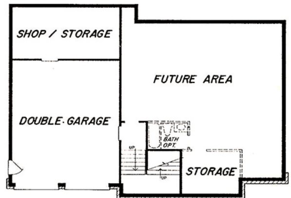
BASEMENT PLAN
