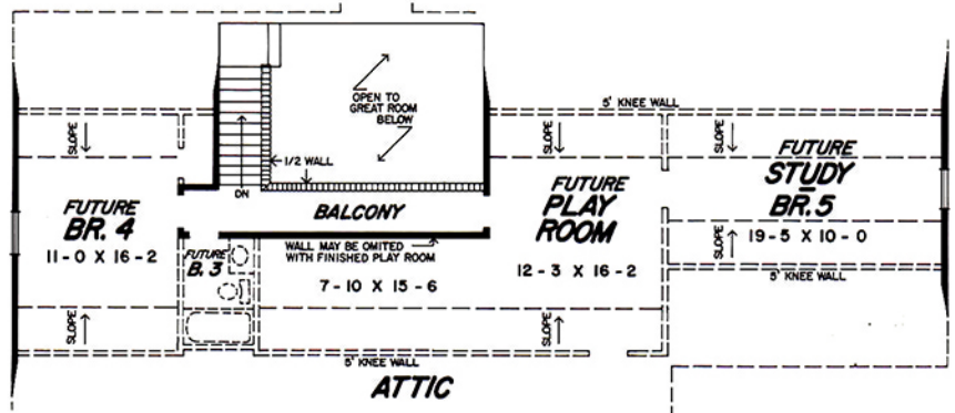
FUTURE SECOND FLOOR PLAN
