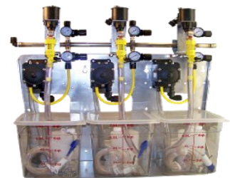
TRIPLE FLOJET PUMP STATION WITH AIR MANIFOLD
