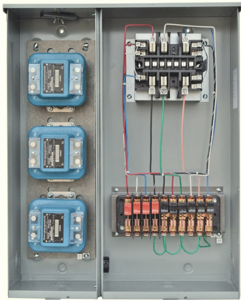
Overhead/Underground Service
