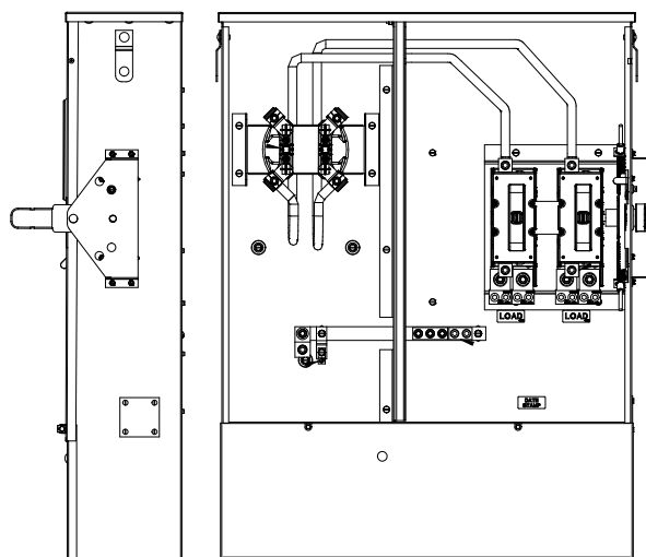
200 Ampere - Pad Mount - 4 Jaw - Self Contained - Ringless Style - Meter Socket/Switches
