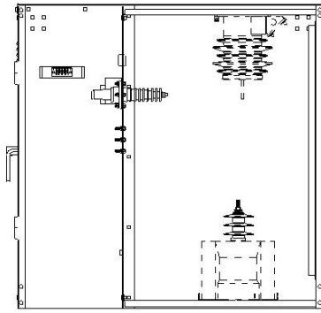
End Section View
