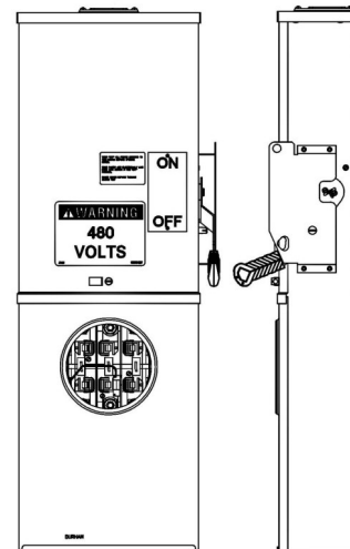
Line Side Cold Sequence Switch
