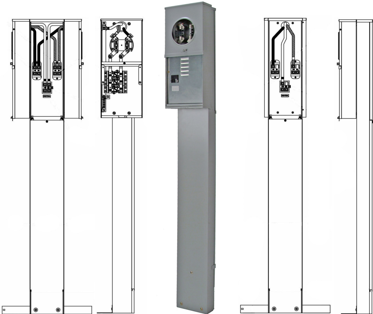
P7911S262W1 200 Amp Plug-In Main Breaker Installed
