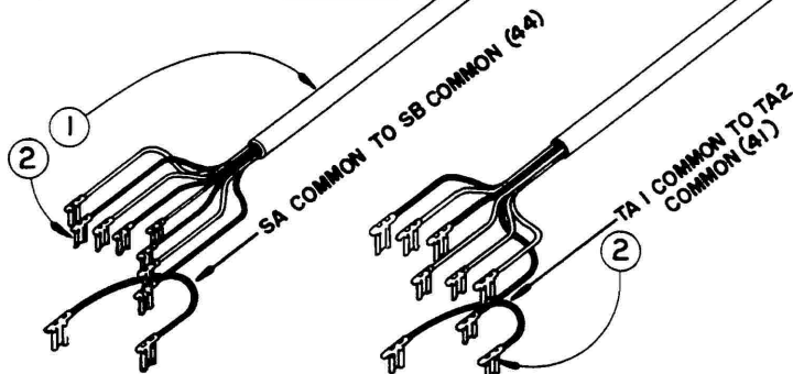
WIRE HARNESS SWEEP CAM SWITCH REFERENCE DRAWING 070 006 452
