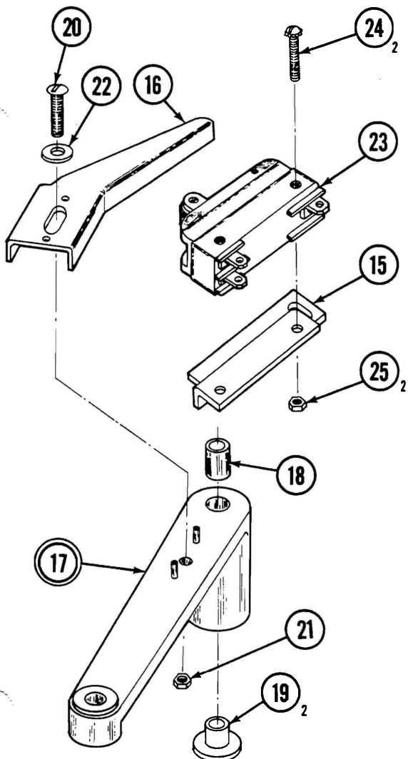
SWITCH & LEVER ASSEMBLY ( 70 A MACHINE TO SERIAL # 93200 )
