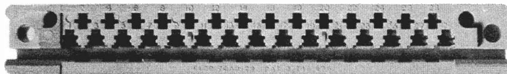
PM and BPP Elco Plug viewed from mating surface with the plug held horizontally with the guide slot down.
