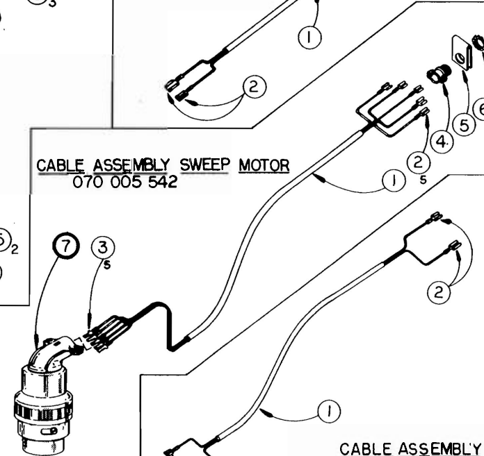
CABLE ASSEMBLY BIN SWITCH (070 006 272)
