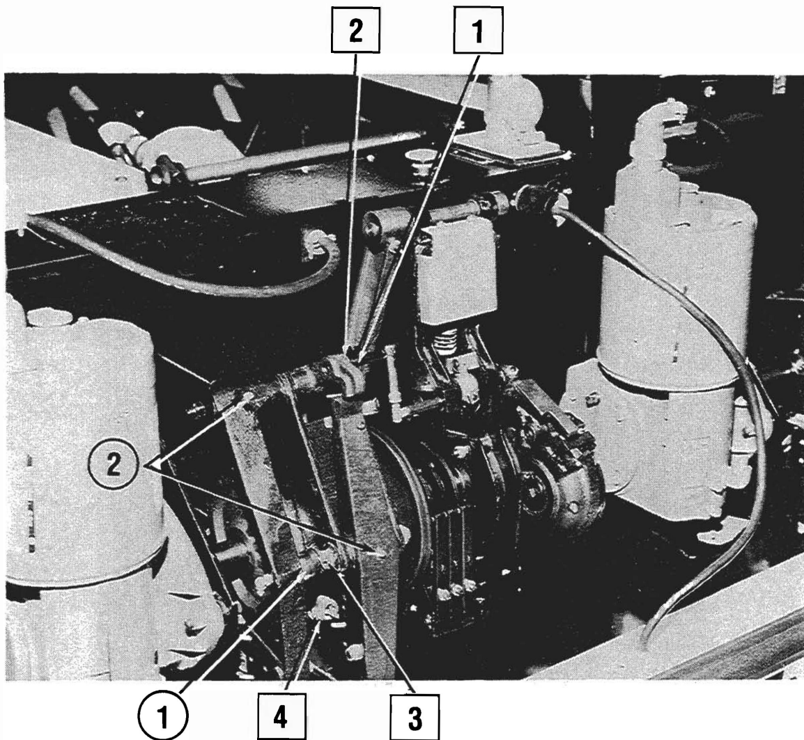
FRONT END ASSEMBLY TABLE TRAVEL CAM LEVERS
