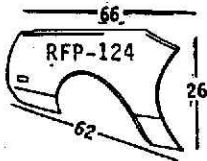
RFP-124 REAR FENDER PANEL, except Fastback
