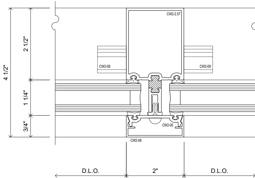
VERTICAL DETAIL
