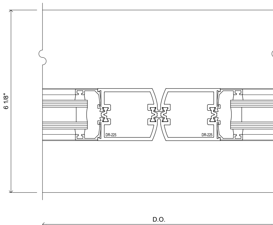
SWING DOOR MEETING STILES DETAIL
