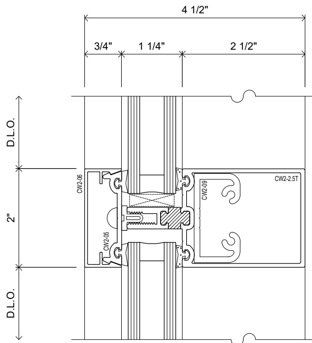
HORIZONTAL DETAIL
