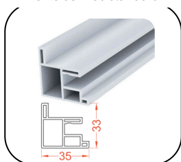
PCR1 Profilo cornice standard
