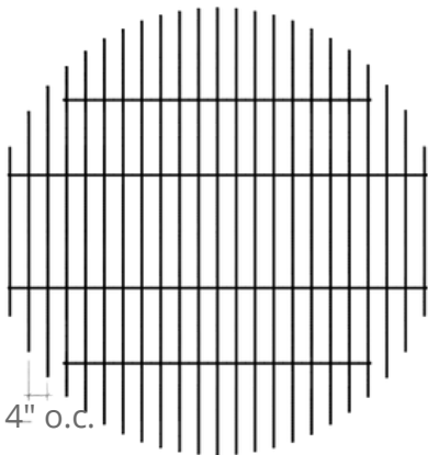
96" Cloud (48" Cloud). 23-Louvers (11-Louvers) 114 Sabins (57 Sabins)
