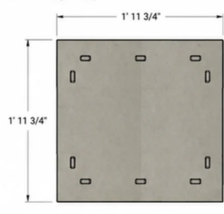
PLAN VIEW (PANEL)
