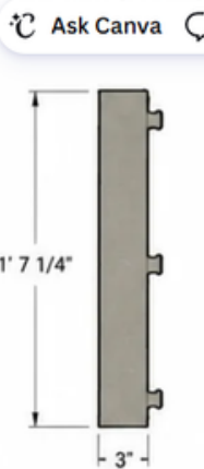
SIDE VIEW (PANEL)
