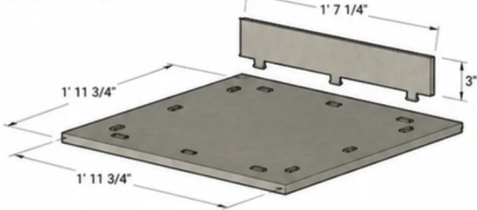
EXPLODED VIEW
