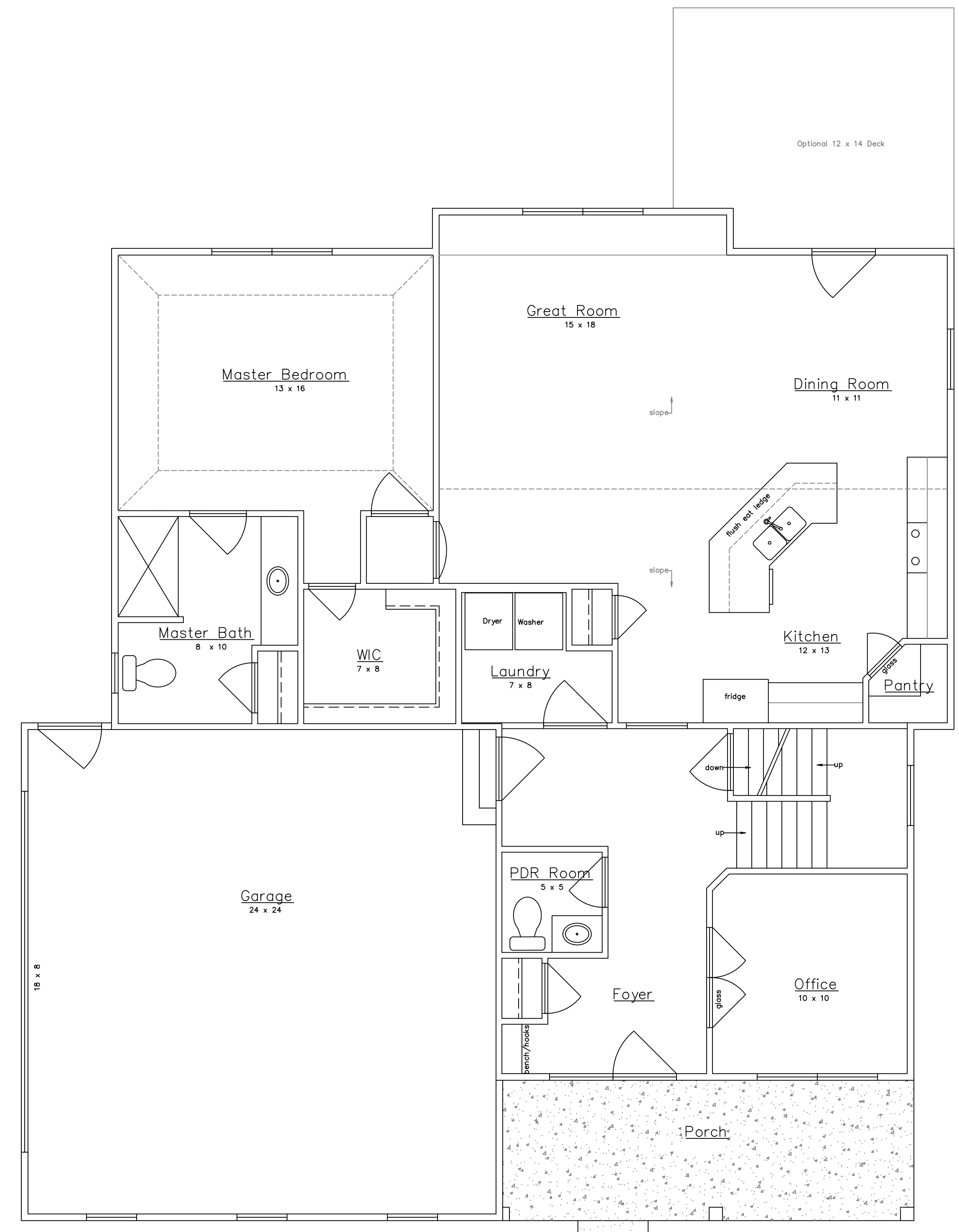
1st Floor plan
