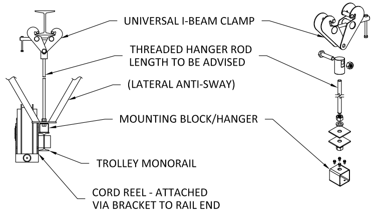
HANGER DETAIL
