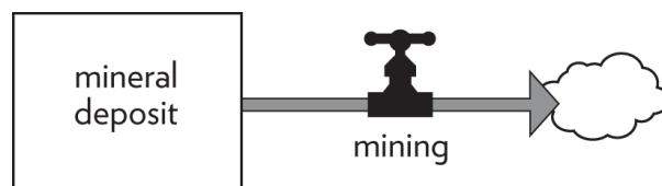
Figure 2. A stock of minerals depleted by mining.
