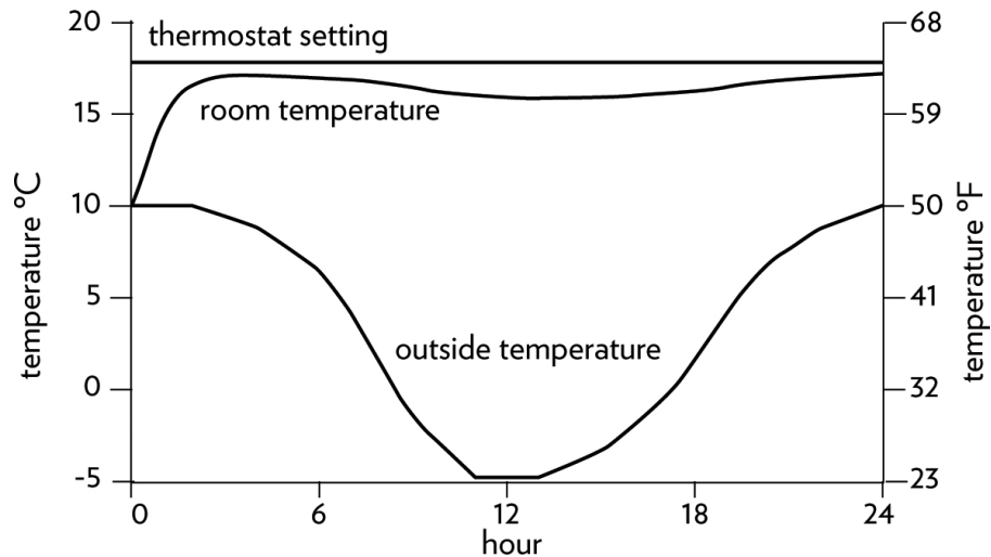
Figure 19. The furnace warms a cool room, even as heat leaks from the room and outside temperatures drop below freezing.
