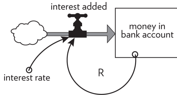
Figure 12. Interest-bearing bank account.
