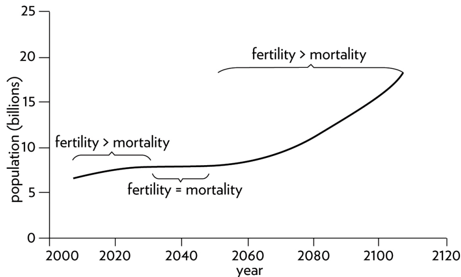
Figure 26. Shifting dominance of fertility and mortality loops.
