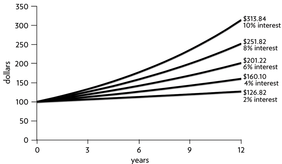
Figure 13. Growth in savings with various interest rates.
