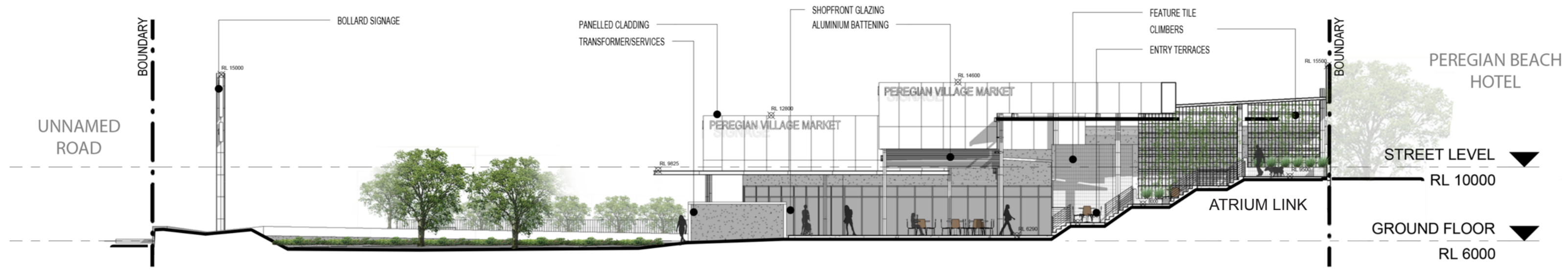
SECTION 1
