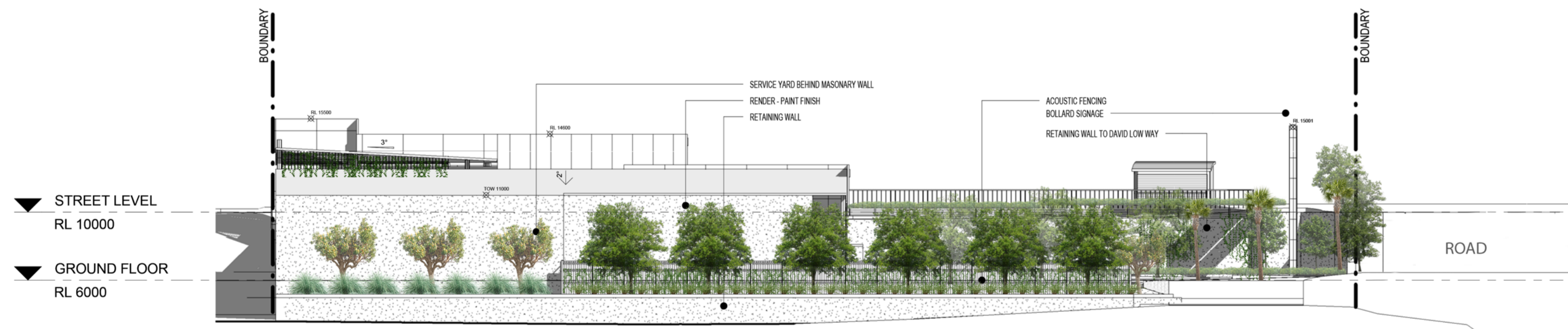
WEST ELEVATION
