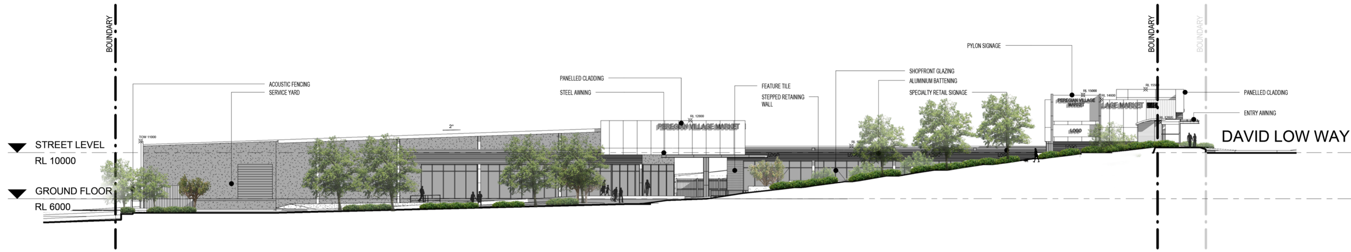
SOUTH ELEVATION
