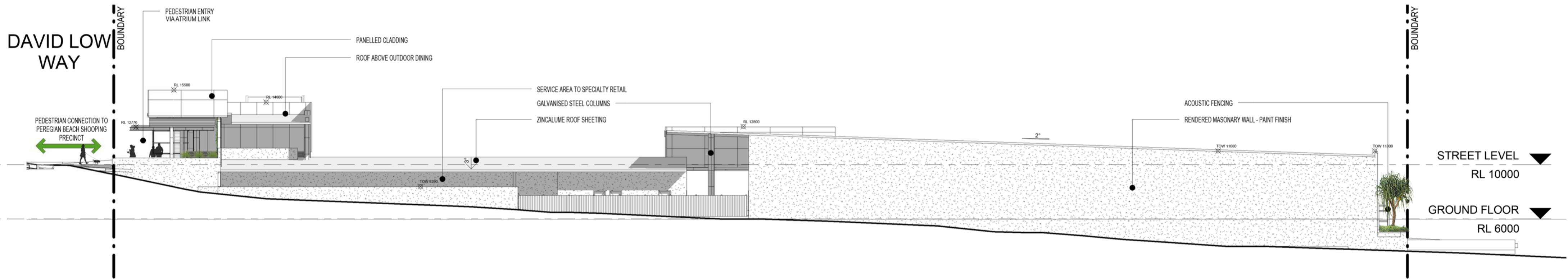
NORTH ELEVATION
