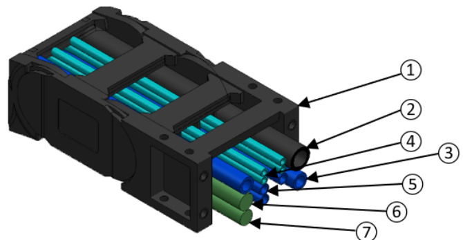
7-D. RAZOR/RAZOR DOUBLE BARREL E-CHAIN
