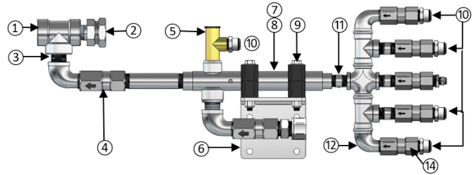
13-A. XR-7 OVERHEAD MANIFOLD
