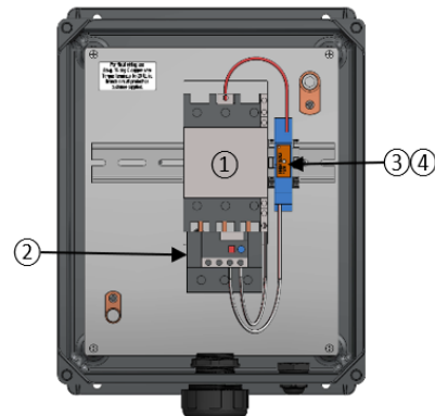
15-D. 25HP MOTOR STARTER
