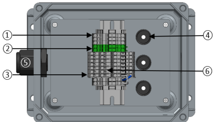
16-C. TROLLEY ENCLOSURE
