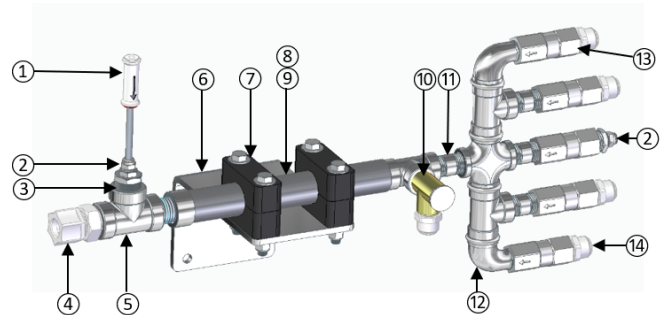
13-B. RAZOR OVERHEAD MANIFOLD
