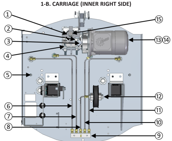
1-B. CARRIAGE INNER RIGHT SIDE
