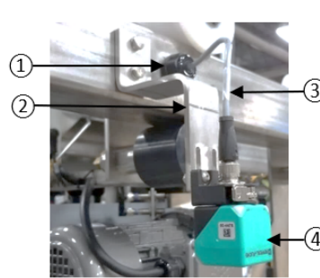
17-D. ↓ REAR ULTRASONIC SENSORS (P&F)
