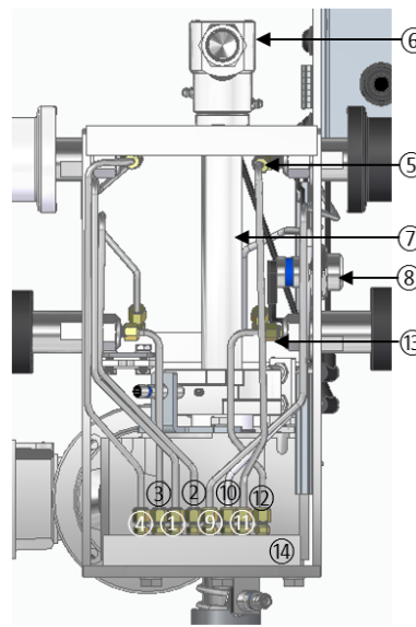
4-A. ↓ RAZOR/XR-7 TROLLEY ASSEMBLY
