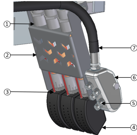
7-A & B. TRI-COLOR FOAM/FLEX PASS HEAD
