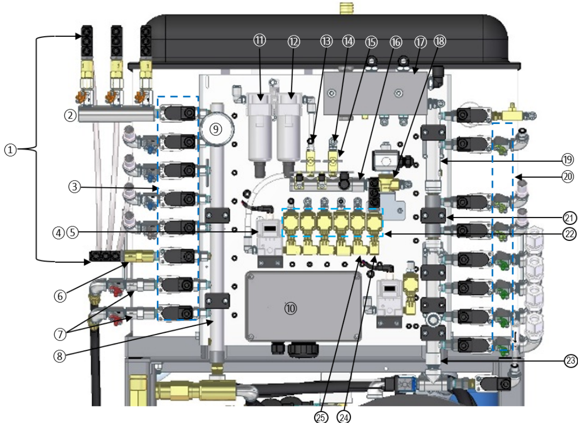
11-A. PUMP STATION PANEL (SN# 61-5440 and above)
