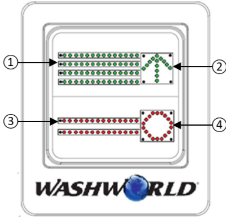
22-A. 24 VAC LED DRIVE FORWARD/WAIT SIGN
