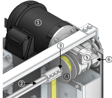
4-B. TOP BRUSH ROLLUP (RIGHT SIDE)
