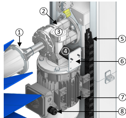
4-D. TOP BRUSH ROTATION (RIGHT SIDE)
