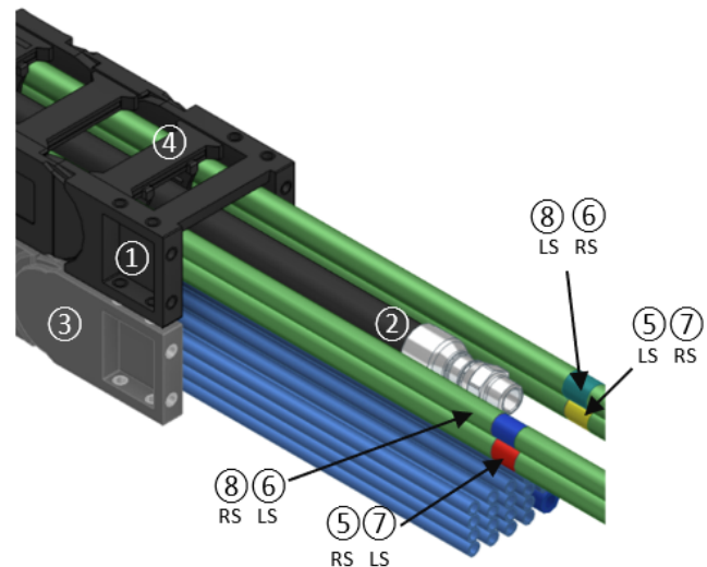
36-C. CARRIAGE E-CHAINS
