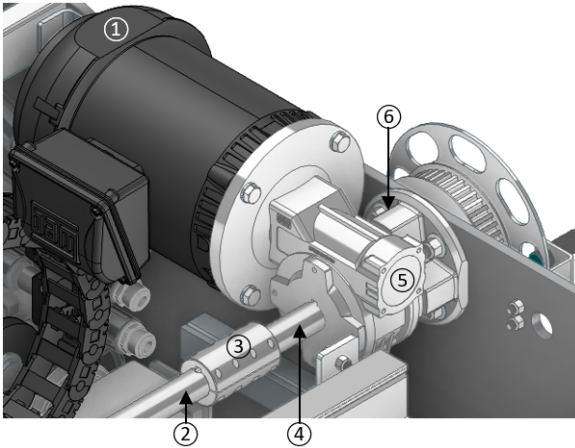
1-B. CARRIAGE DRIVE
