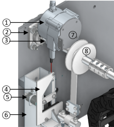
33-A. TOP ARCH ROLLUP (LEFT SIDE)
