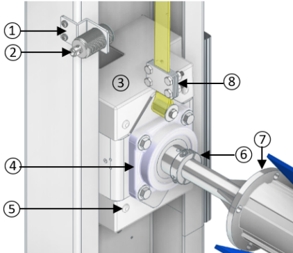
4-C. TOP BRUSH ROTATION (LEFT SIDE)
