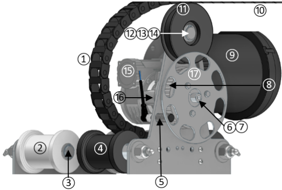
3-A. SIDE BRUSH TROLLEY (UPPER HALF)
