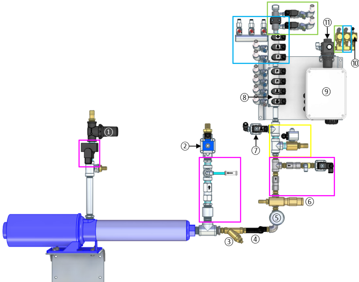
28-C. LXR LOW PRESSURE PUMP & PANEL
