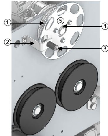
1-C. CARRIAGE DRIVE
