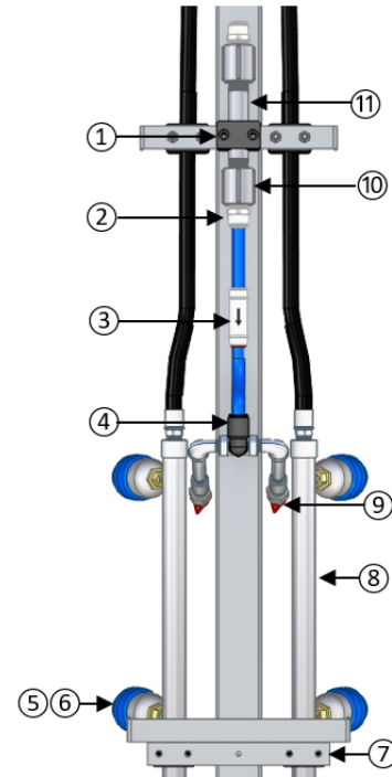
6-B. SIDE ARM FLUID CONNECTIONS
