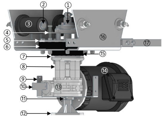
3-B. SIDE BRUSH TROLLEY (LOWER HALF)
