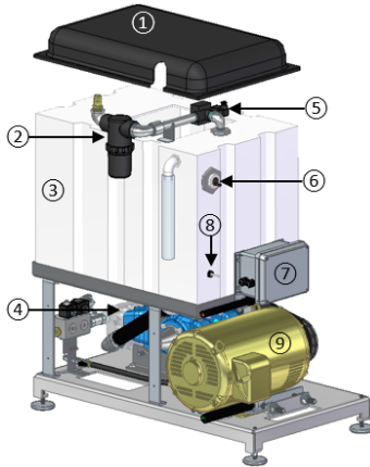
14-A. HIGH PRESSURE STAND
