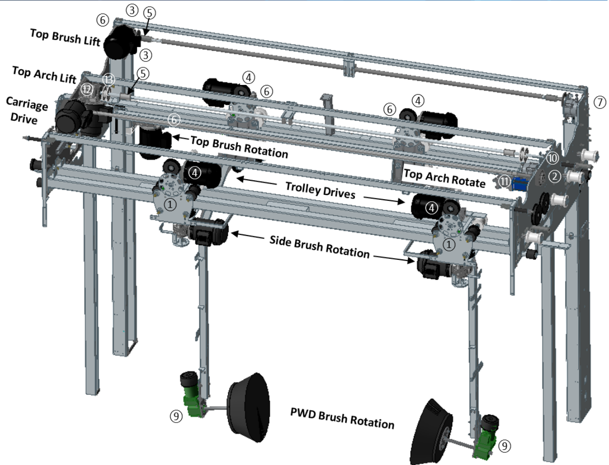
PROFILE/APEX/LXR - MOTOR/GEARBOX AND KEY REFERENCE CHART
