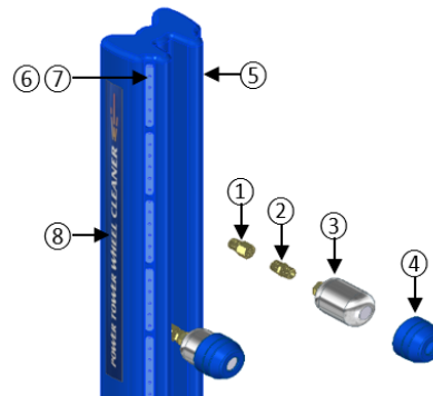
25-C. POWER TOWER WHEEL CLEANER
