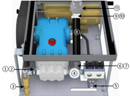
14-B. HIGH PRESSURE PUMP
