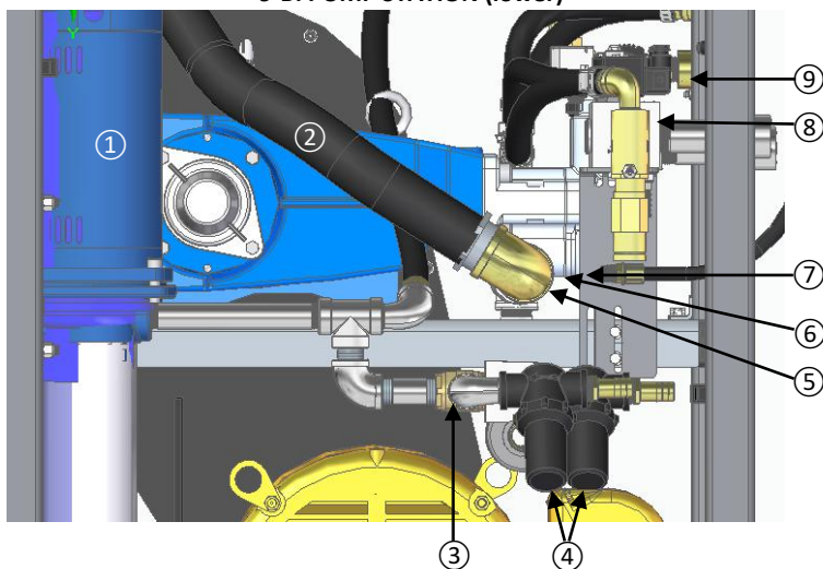
9-B. PUMP STATION (lower)
