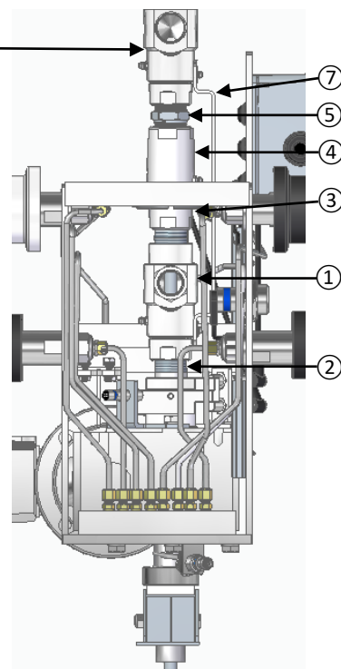
DOUBLE BARREL TROLLEY ASSEMBLY
