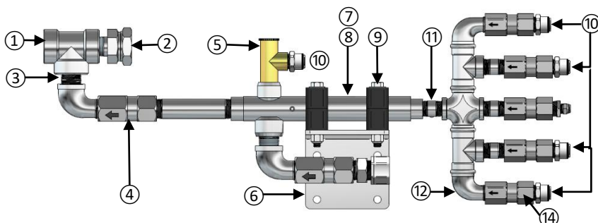
12-B. RAZOR OVERHEAD MANIFOLD (SN# 60-5589 and above)
