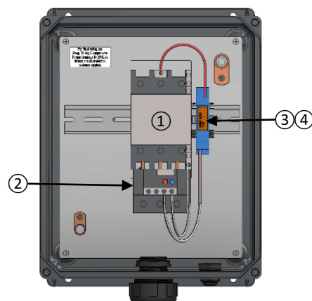
14-D. 25HP MOTOR STARTER
