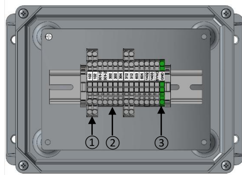
14-C. VS2 ENCLOSURE
