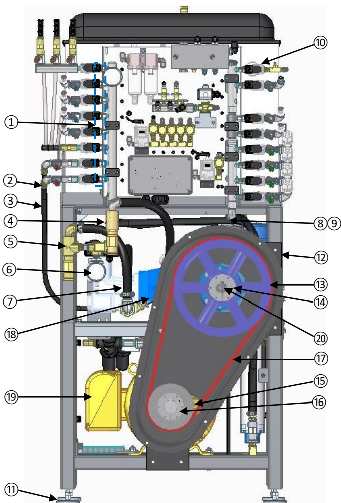
9-A. PUMP STATION (SN# 60/61-3050 and above)
