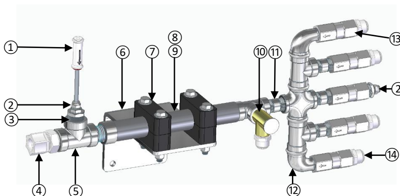
12-B. RAZOR OVERHEAD MANIFOLD (SN# 60-5589 and above)
