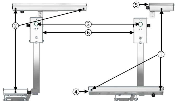
27-C. RIGHT & LEFT-SIDE LOADING EYES
