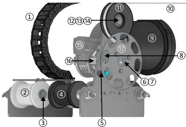
3-A. SIDE BRUSH TROLLEY (UPPER HALF)
