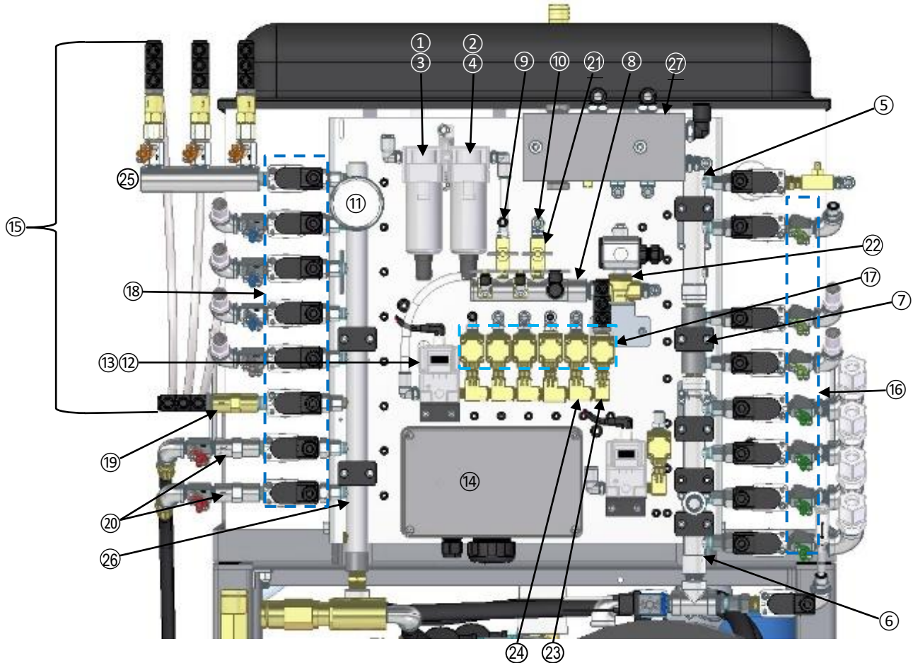
10-A. PUMP STATION PANEL (SN# 61-5440 and above)
