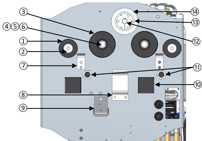
1-A. CARRIAGE (OUTER RIGHT SIDE)
