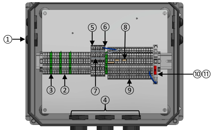
15-B. CARRIAGE ENCLOSURE
