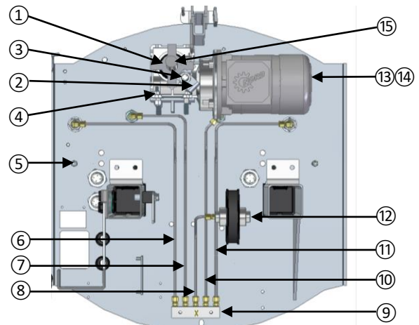
1-B. CARRIAGE (INNER RIGHT SIDE)
