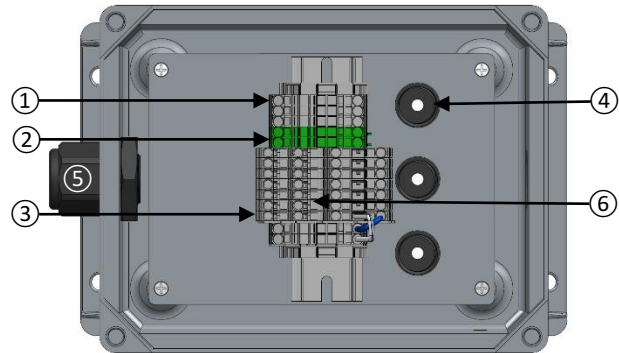
15-C. TROLLEY ENCLOSURE
