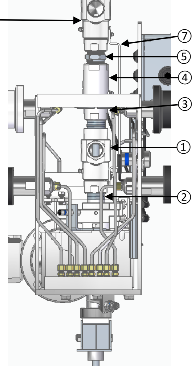
DOUBLE BARREL TROLLEY ASSEMBLY
