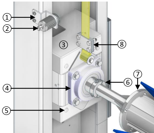
4-C. TOP BRUSH ROTATION (LEFT SIDE)
