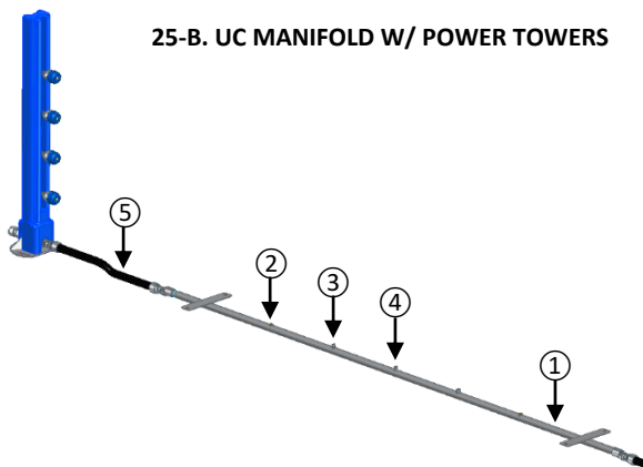
25-B. UC MANIFOLD W/ POWER TOWERS
