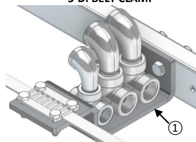
5-D. BELT CLAMP
