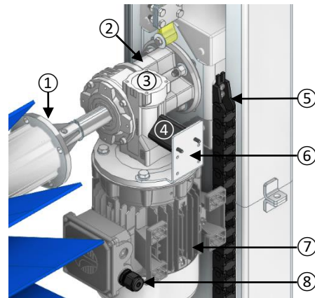
4-D. TOP BRUSH ROTATION (RIGHT SIDE)
