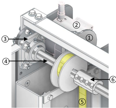
4-A. TOP BRUSH ROLLUP (LEFT SIDE)
