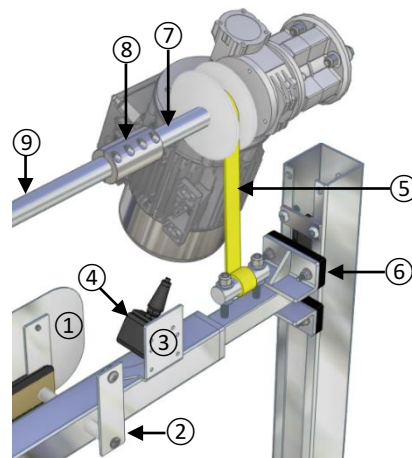
34-B. TOP ARCH ROLLUP (RIGHT SIDE)
