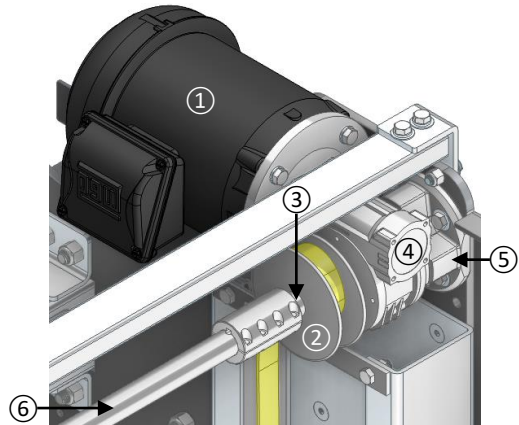
4-B. TOP BRUSH ROLLUP (RIGHT SIDE)
