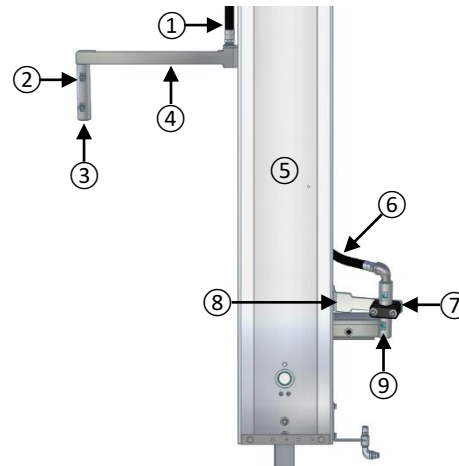
27-C. RIGHT & LEFT-SIDE LOADING EYES
