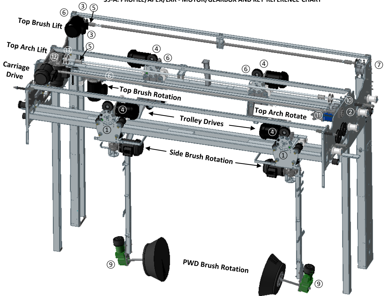
39-A. PROFILE/APEX/LXR - MOTOR/GEARBOX AND KEY REFERENCE CHART
