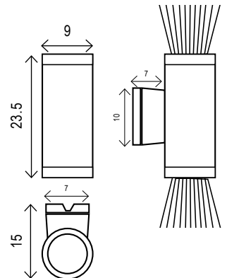
Metro GU10 Twin
