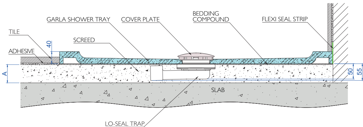
DIMENSION A: MIN - 50mm (Assumes outlet is directly next to SVP) DRAWN AS: 60mm
