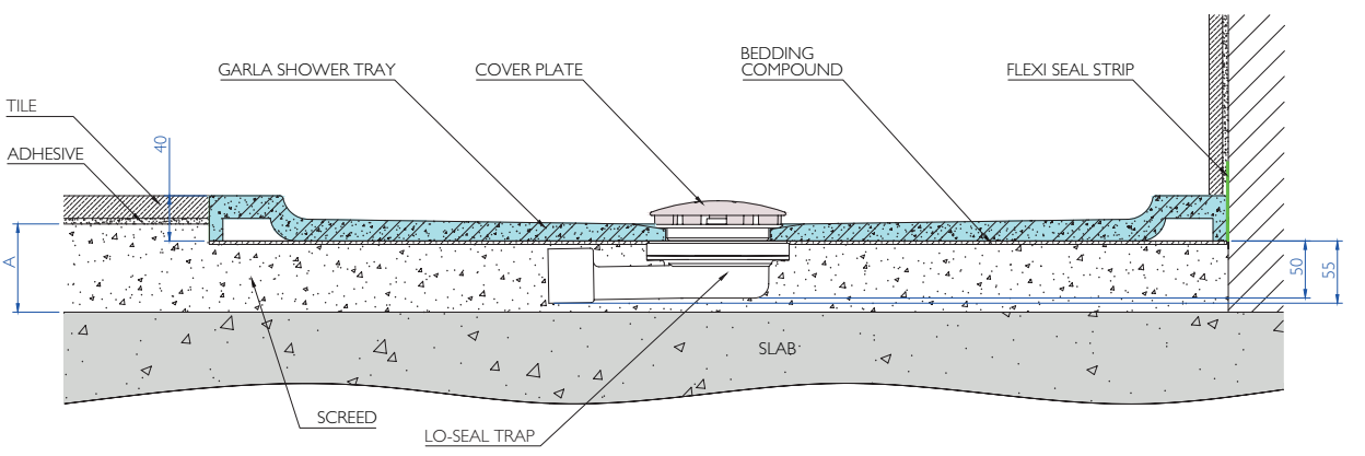
DIMENSION A: MIN - 50mm (Assumes outlet is directly next to SVP) DRAWN AS: 60mm
