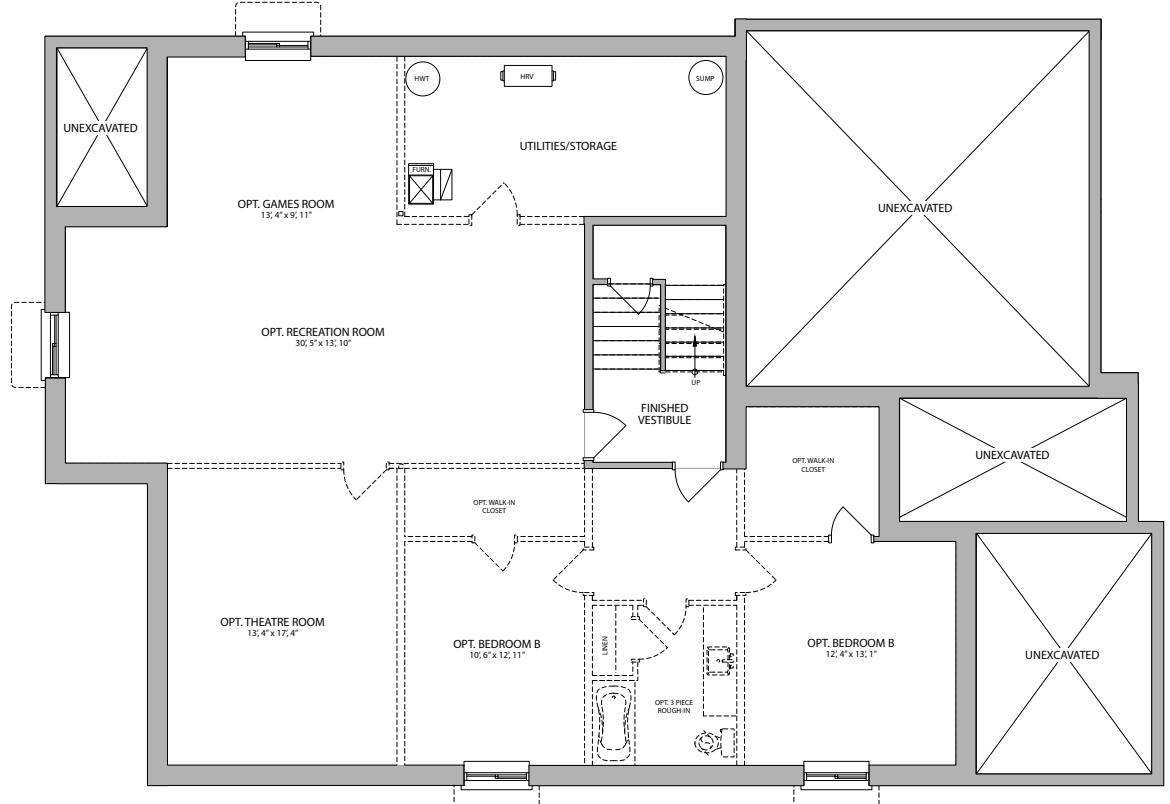
BASEMENT FLOOR PLAN Elevation A & B
