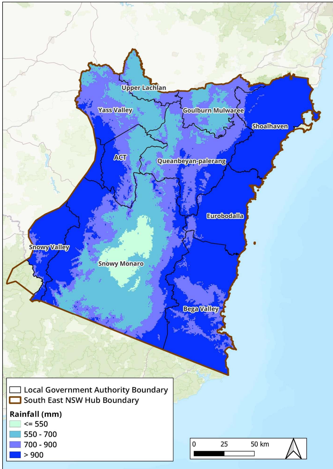
Figure 5-2: Input – Rainfall
