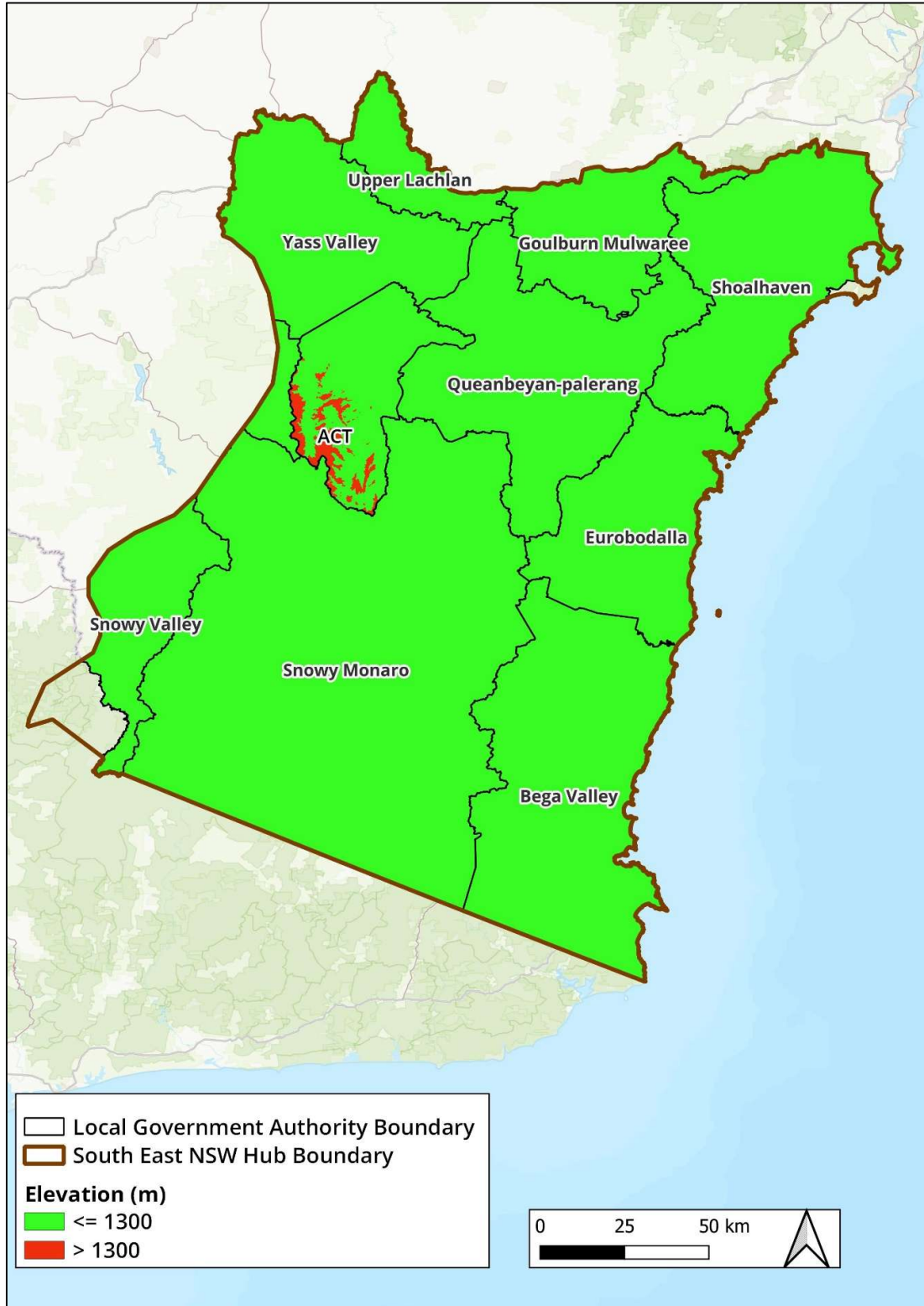
Figure 5-1: Input – Elevation
