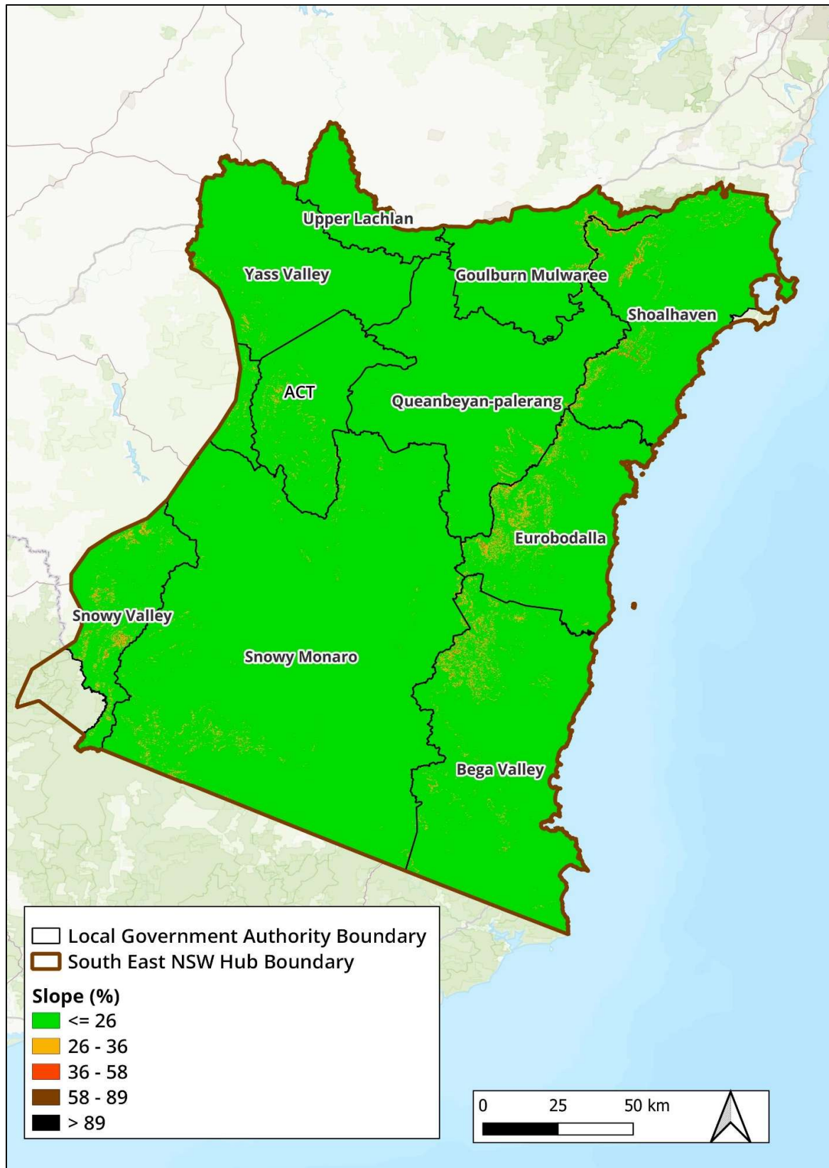
Figure 5-3: Input – Slope
