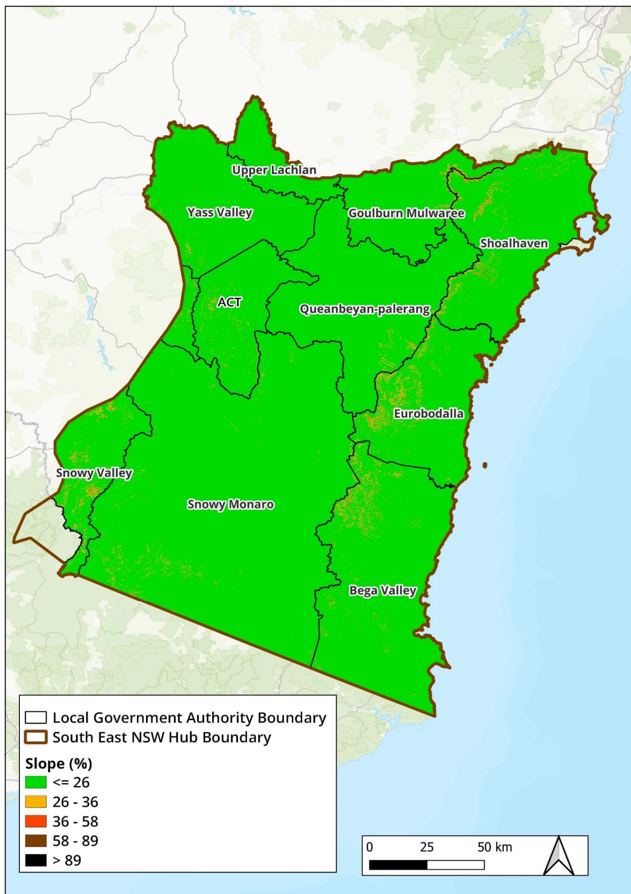
Figure 5-3: Input – Slope
