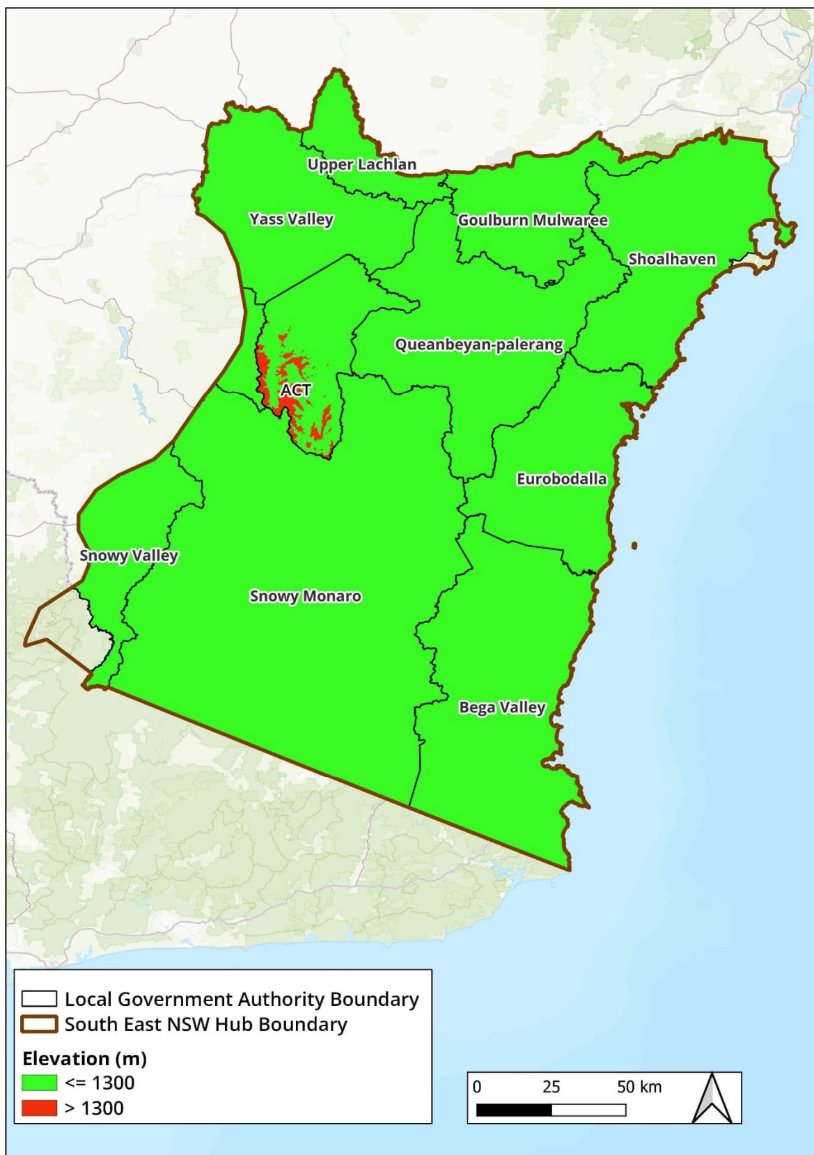
Figure 5-1: Input – Elevation
