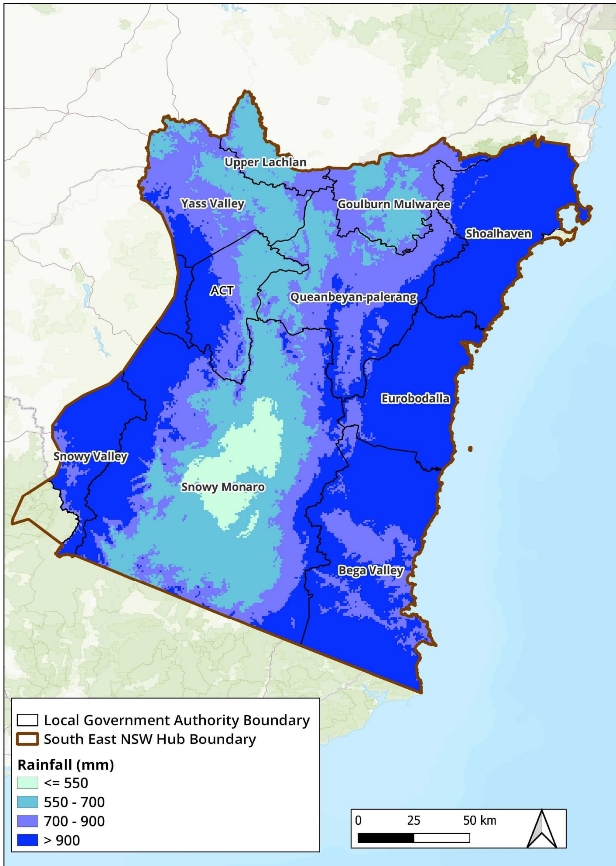
Figure 5-2: Input – Rainfall
