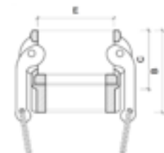
800-02858 POLY CAMLOCK D. FEMALE COUPLING TO FBSP THREAD 25MM
