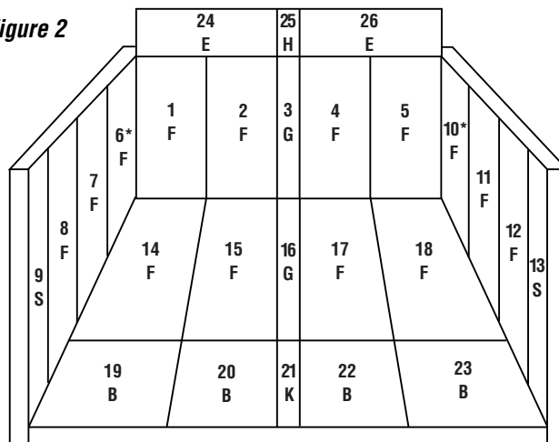
Firebox Brick Layout Viewed From the Front
