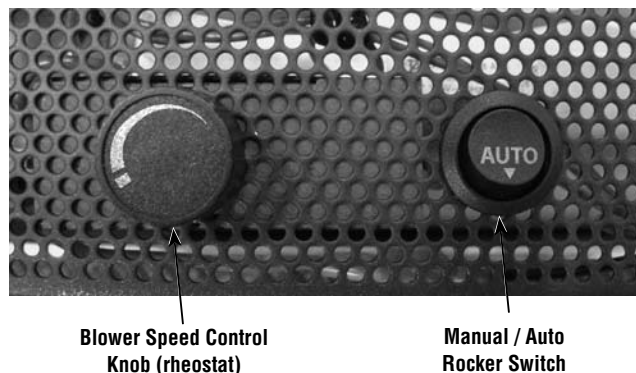
Figure 11 - Blower Controls
