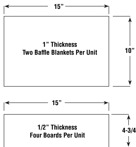
Baffle Insulation Parts
