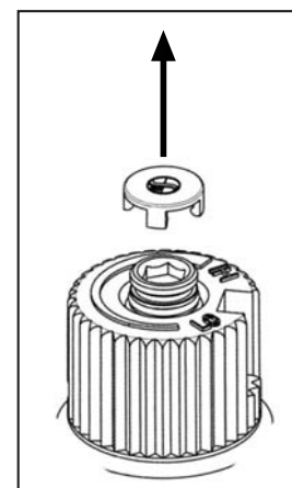
Figure 11: Removing valve cap.
