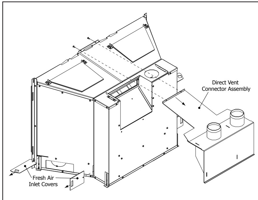
Figure 25: Converting to a BV fireplace.
