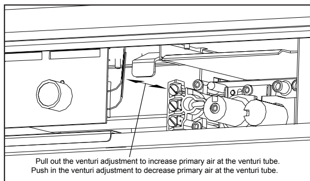
Figure 7: Adjusting the venturi air setting.
