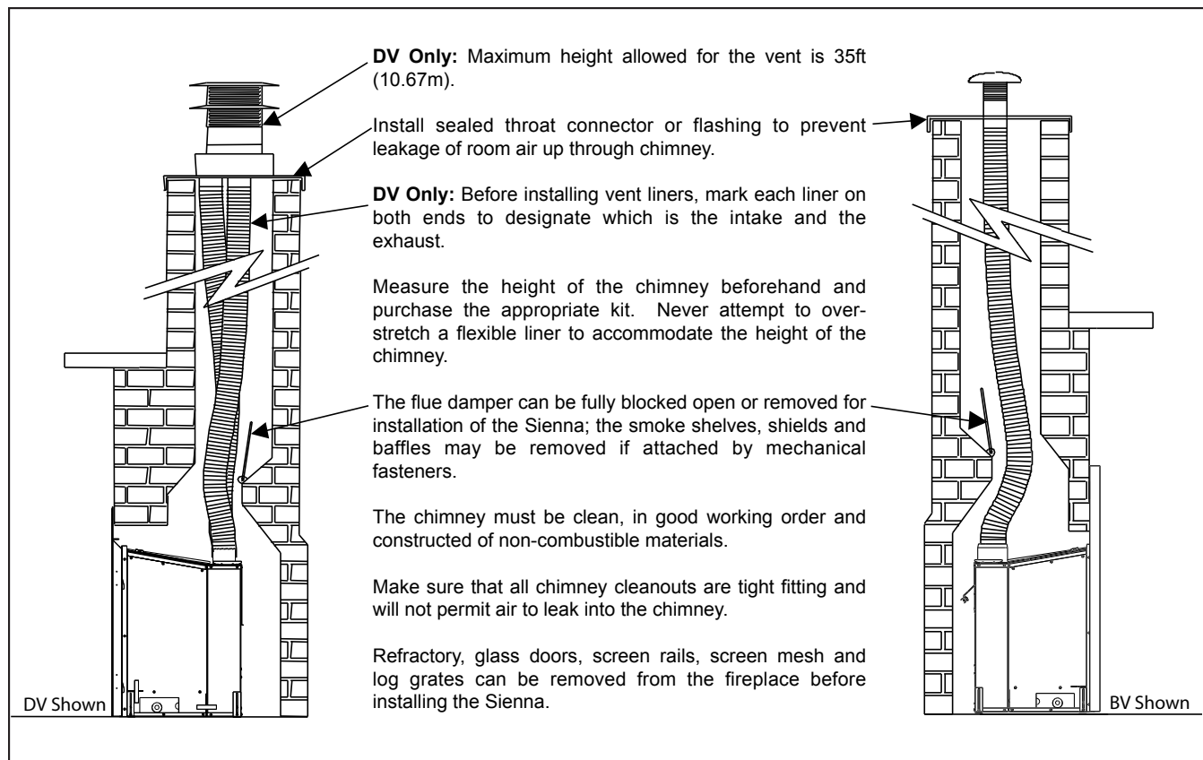
Figure 20: Installation of Sienna DV and BV.
