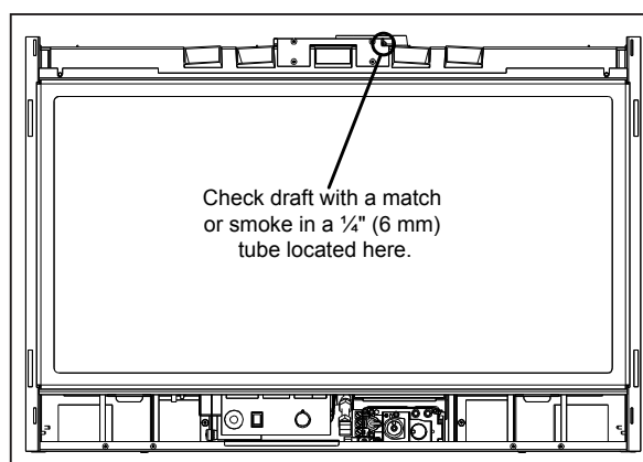
Figure 18: Draft check.
