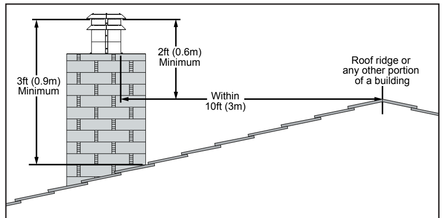
Figure 21: Roof Clearances.
