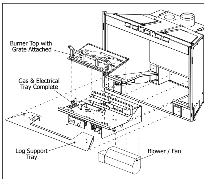
Figure 10: Removing burner and gas tray.
