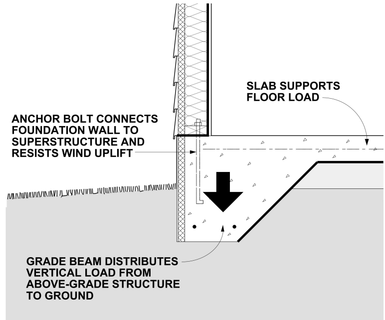
Figure 4-2: Structural Components of Slab-on-Grade Foundation with Grade Beam
