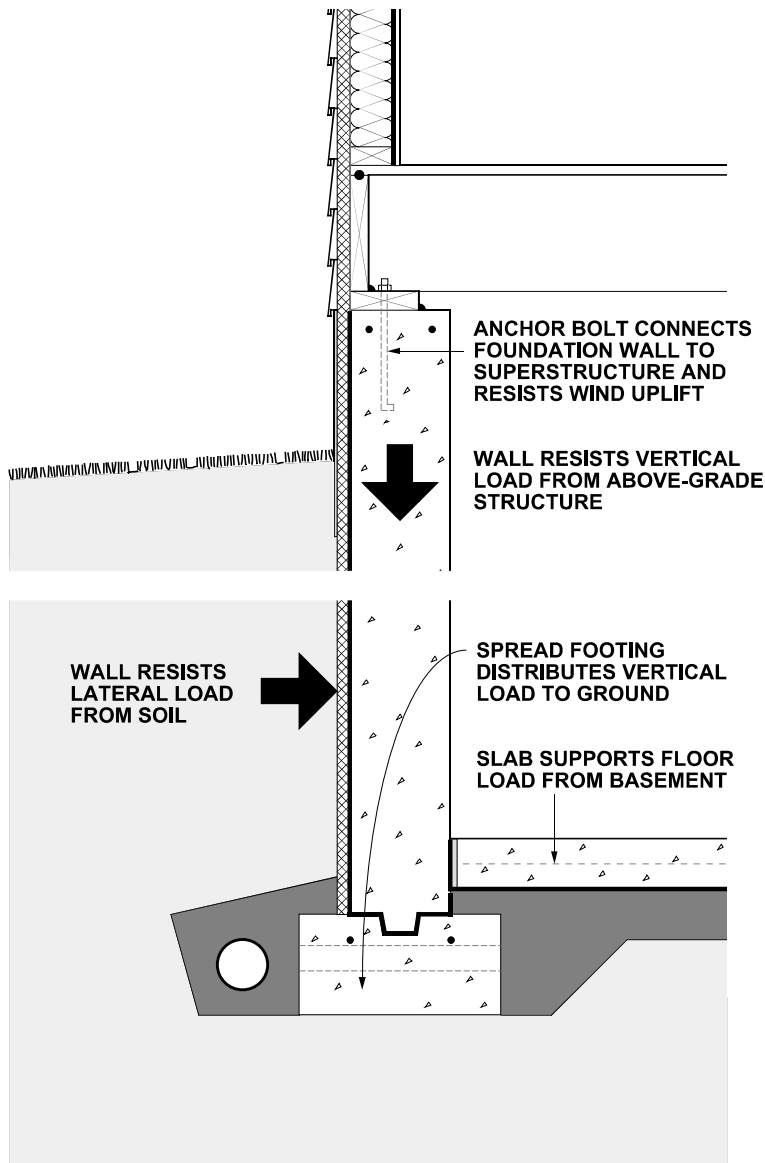
Figure 2-2: Components of Basement Structural System
