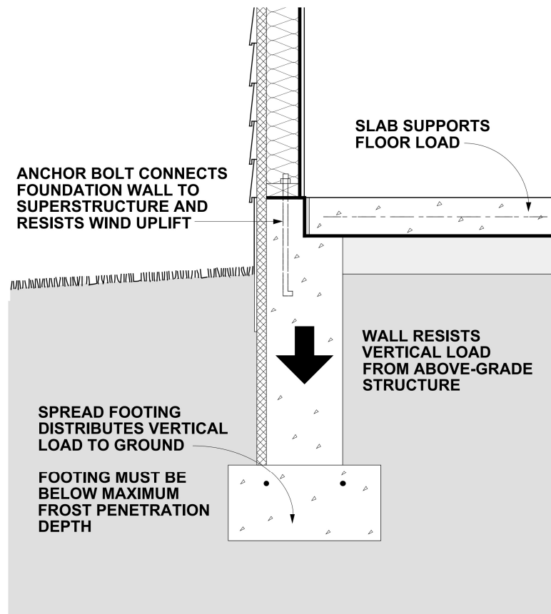
Figure 4-3: Structural Components of Slab-on-Grade Foundation with Stem Wall and Footing
