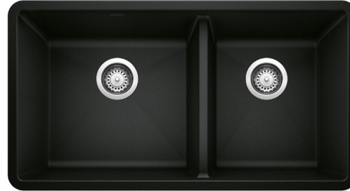
Precis 60/40 UM OD: 33" W X 18" D X 10" H L: 17" W X 16" D X 9 1/2" H R: 13" W X 16" D X 9 1/2" H
