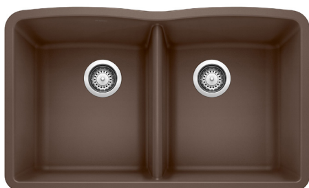
Diamond 50/50 UM OD: 32" W X 19 1/4" D X 10" H L: 14 1/2" W X 17" D X 9 1/2" H R: 14 1/2" W X 17" D X 9 1/2" H
