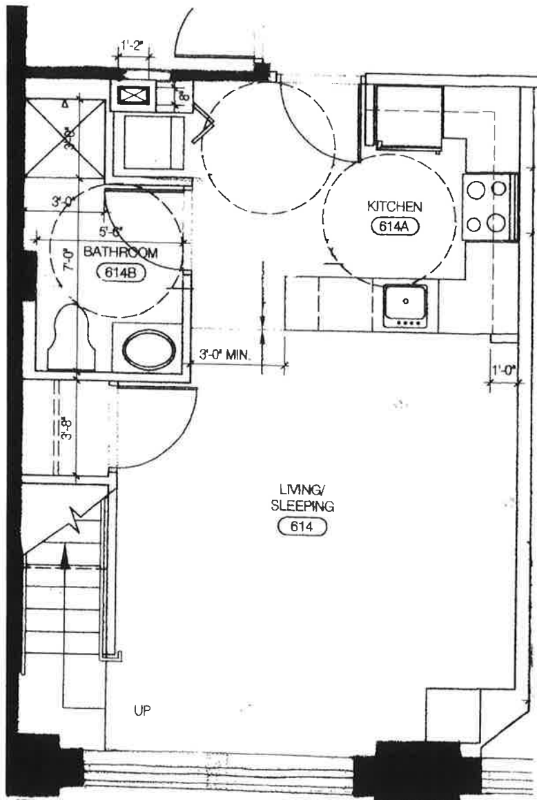
UNIT FLOOR PLANS - 614 (LOWER FLOOR)
